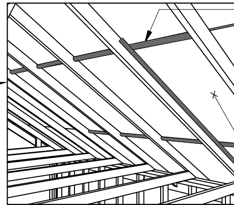
UNDERSIDE OF ROOF DECK FROM WITHIN ATTIC
